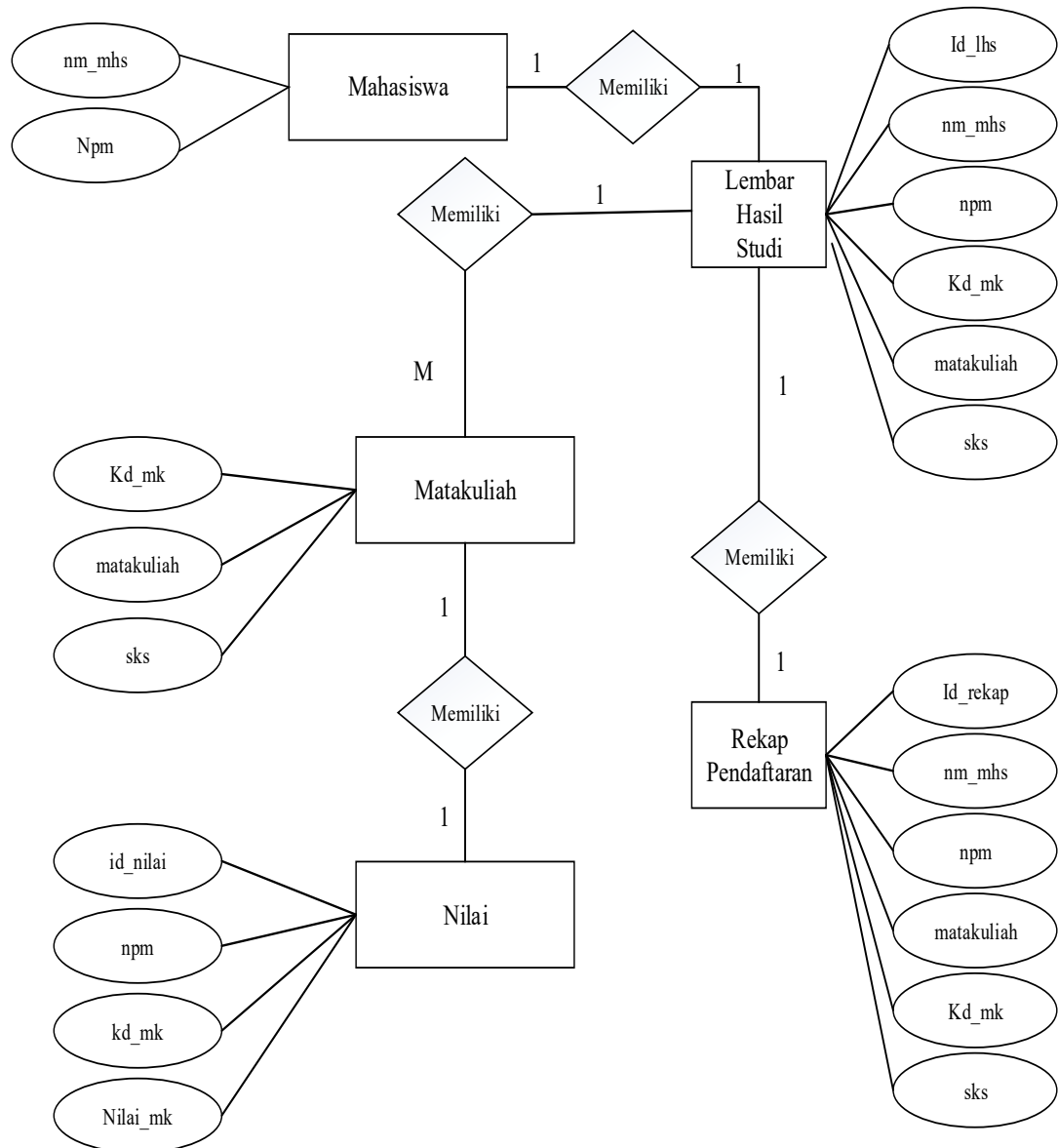
Gambar 3.4 Entity Relationship Diagram
