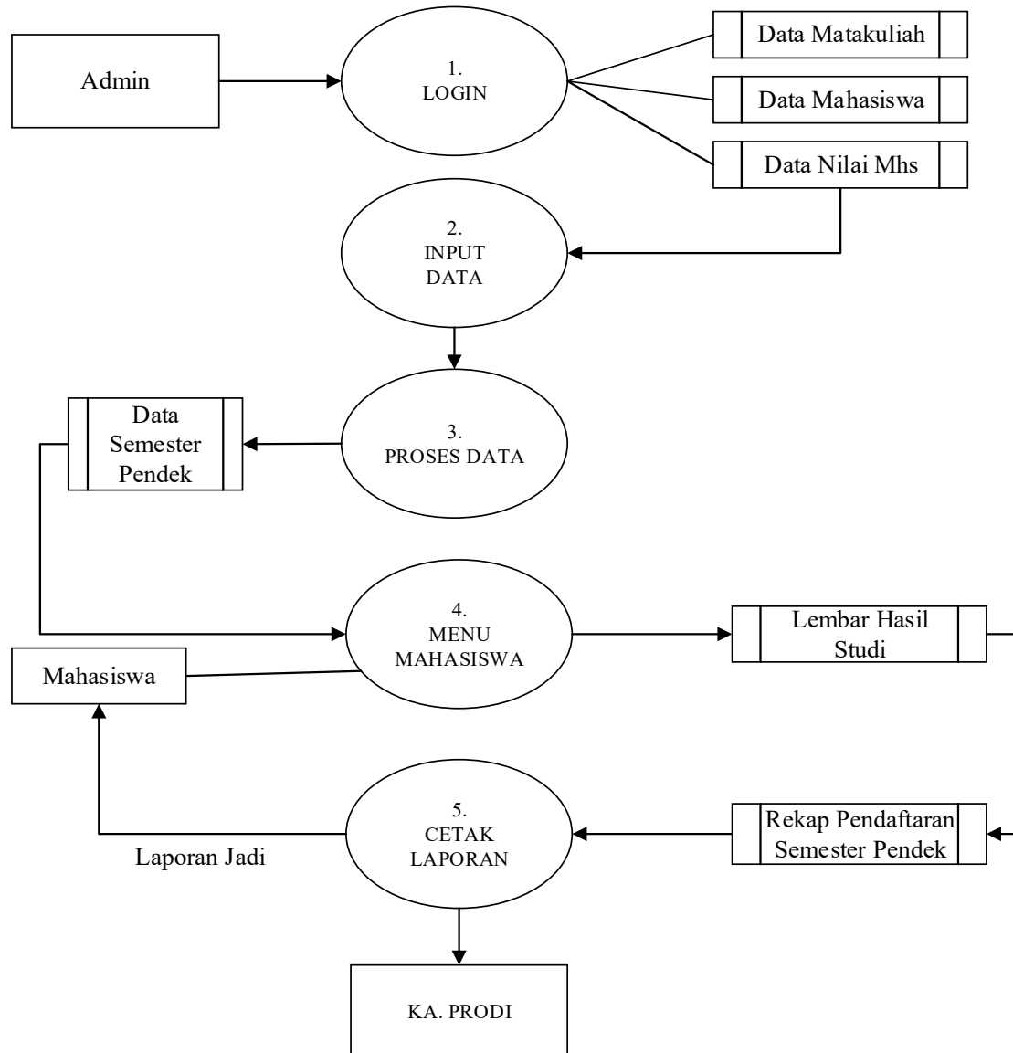
Gambar 3.3 DFD level 1
